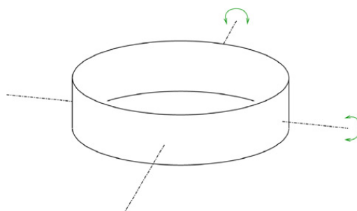
Fig. 3. The action of \mathbf{Z}/2 \oplus \mathbf{Z}/2 on the annulus A_i .
