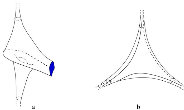
Fig. 6. An annulus and two ideal triangles.
