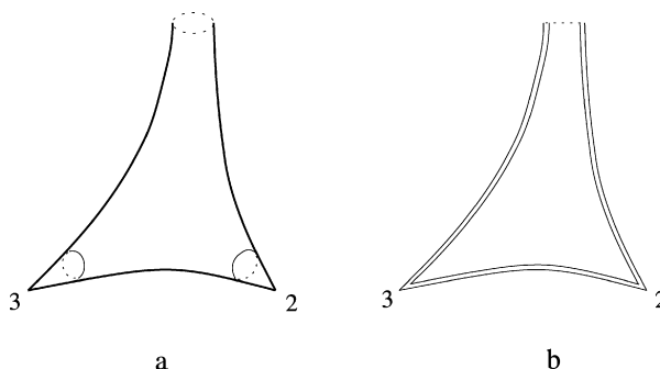
Fig. 4. The possible quotients of P . Case b is non-orientable, has mirror points (double lines), and corners.
