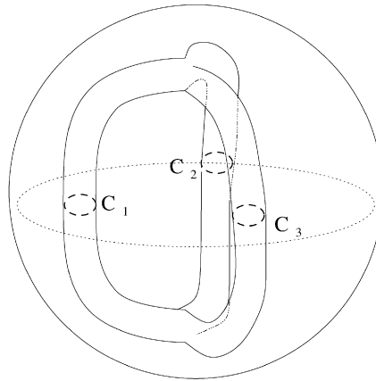
Fig. 1. The handlebody H contained in a ball and the three curves C_i .
