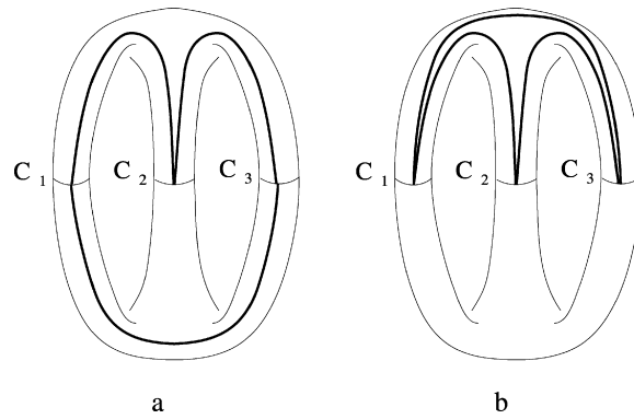
Fig. 7. The intersection \varphi(P_j) \cap (P_1 \cup P_2) , viewed in \partial H = P_1 \cup P_2 \cup \bigcup_{i=1}^3 C_i .
