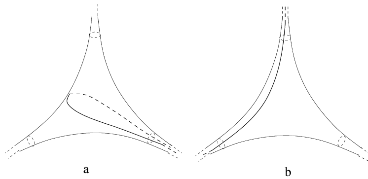
Fig. 5. The two types of geodesic intersections.
