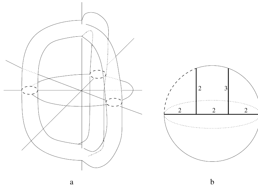
Fig. 2. The group \mathbf{Z}/2 \times \mathbf{D}_3 acting on H and the quotient orbifold \mathcal{O} .
