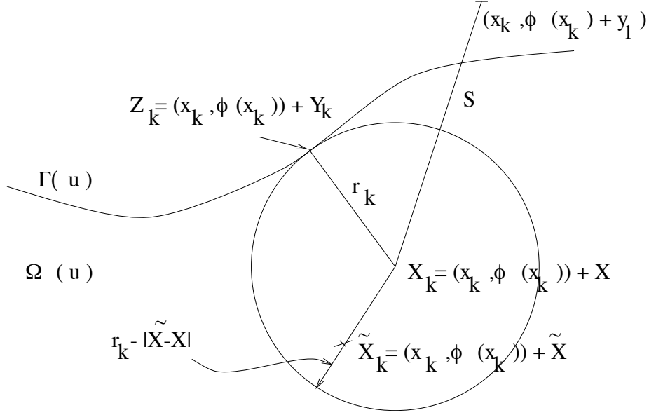
Figure 2: The ball of radius r_k and center X_k
