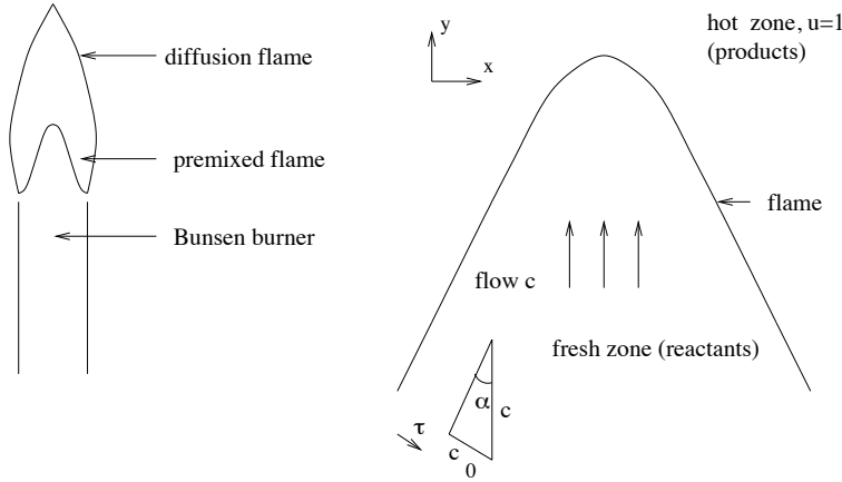
Figure 1: Bunsen flames, the premixed flame
