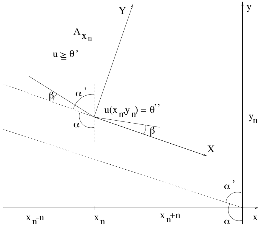
Figure 1: The set \mathcal{A}_{x_n}
